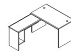
STANDARD TABLE/1.2-6 T120 - 1200W*1700D*750H
