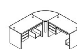
STANDARD TABLE/1.2-8 T120 - 1900W*1900D*750H
