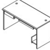
STANDARD TABLE/1.4-3 T140 - 1400W*700D*750H
