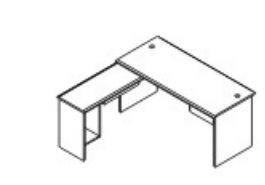
STANDARD TABLE/1.6-7 T160 - 1600W*1700D*750H
