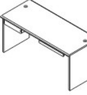
STANDARD TABLE/1.6-2 T160 - 1600W*700D*750H
